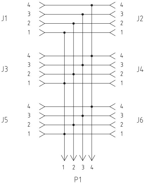
WIRING DIAGRAM
